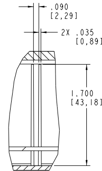
DETAIL C SCALE 2:000 TYP PCB SUPPORT RIB DESIGN
